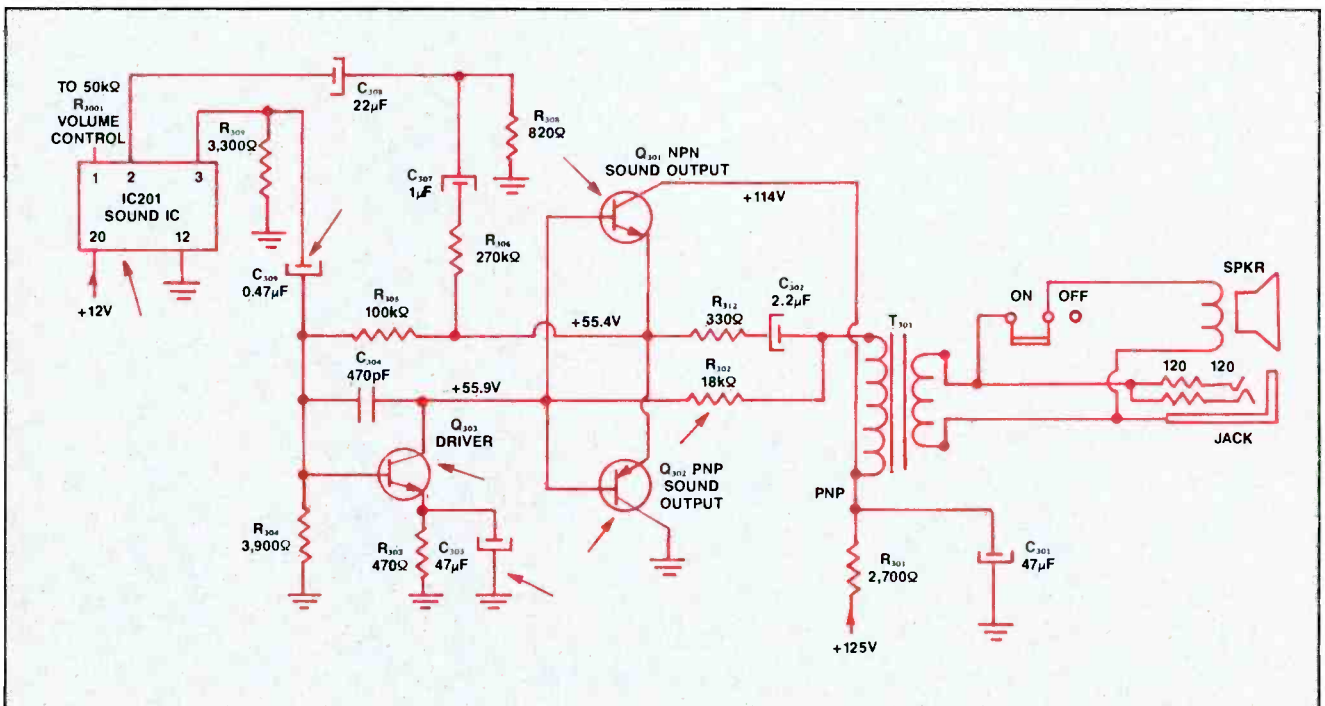
Figure 2. Try the easy things first is good troubleshooting advice for a 9H100 audio circuit without sound or with low-volume sound: measure the dc voltage at Q_{301} 's collector, expecting a normal +114V . Low voltage there must be investigated and the cause repaired. Past experience shows that distorted sound often is caused by a defective Q_{301} , Q_{302} , R_{302} or IC201.
